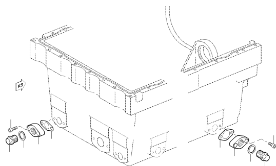
SEAL ELEM. 010.00141
