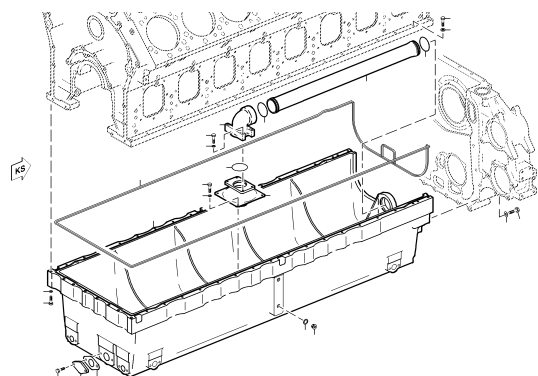
OIL PAN 010.00084
